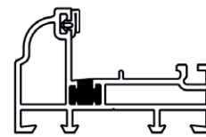
44MM ALUMINIUM THRESHOLD (OVOLO)
